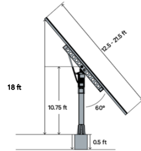
Fig. 2. Schematic of tracker dimensions depicts vertical height of the tracker platform, which adds light to the backside, an amount that increases with tilt angle.
